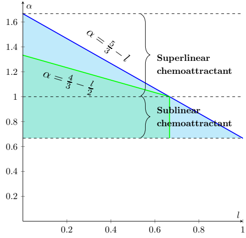
(B) Case n = 3 . PP: l \in (0, \frac{2}{3}) , \frac{2}{3} \leq \alpha < \frac{4}{3} - \frac{l}{2} . PE: l \in (0, 1) , \frac{2}{3} \leq \alpha < \frac{5}{3} - l .
